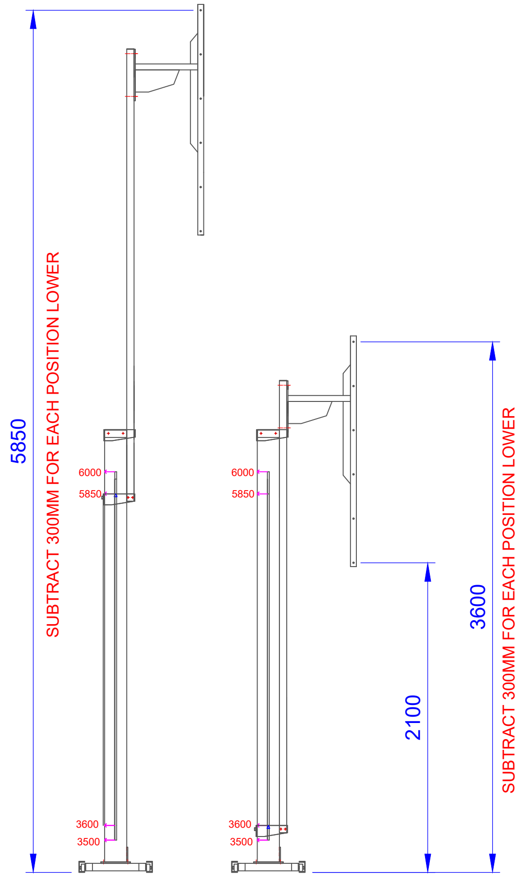
TPV60 POLE VAULT STAND ASEEMBLY
